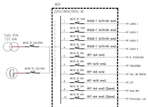
Gambar 2. Single Line Diagram Panel MDP
